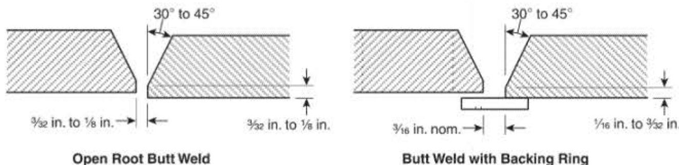
FIGURE A.4.4.2.2 Weld Diagram.
