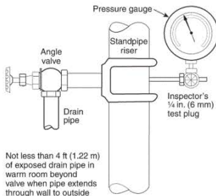
FIGURE 7.11.2.1 Drain Connection for System Riser.
