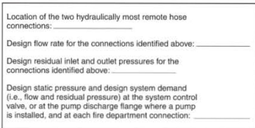
FIGURE A.6.8 System Hydraulic Design Information Sign.
