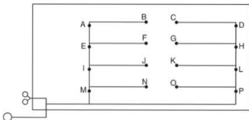
FIGURE A.7.10.1.1.6 Standpipe System with Single Hose Connections Served by a Lateral Pipe.
