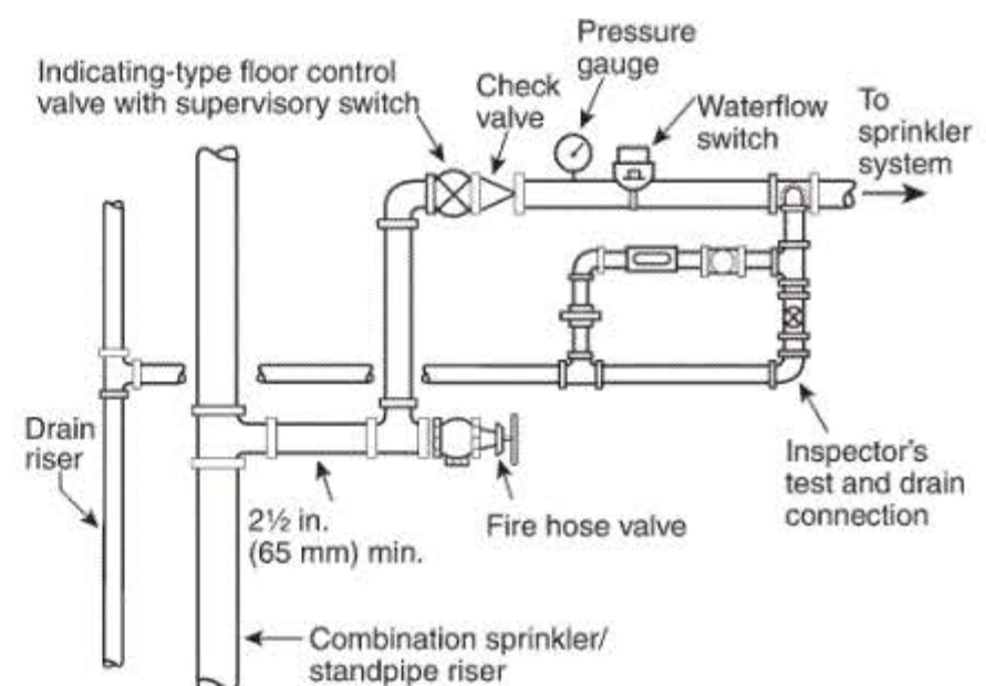
FIGURE A.6.3.5(b) Combined Sprinkler/Standpipe System.
