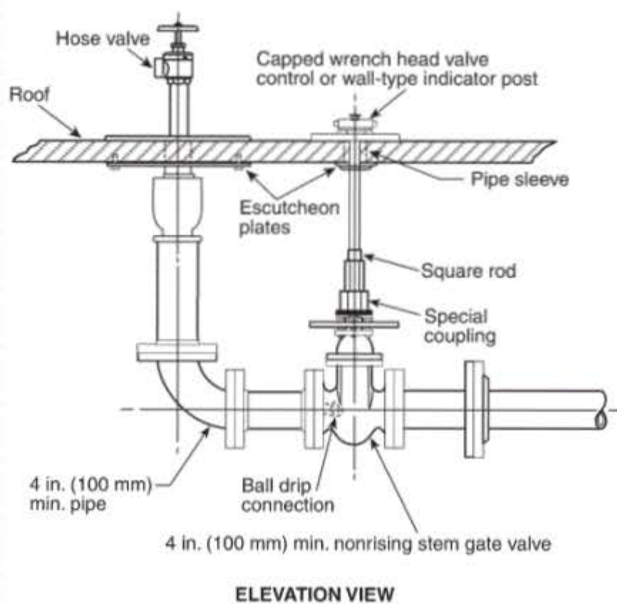
FIGURE A.7.3.2.7 Roof Hose Connection Piping Arrangement.
