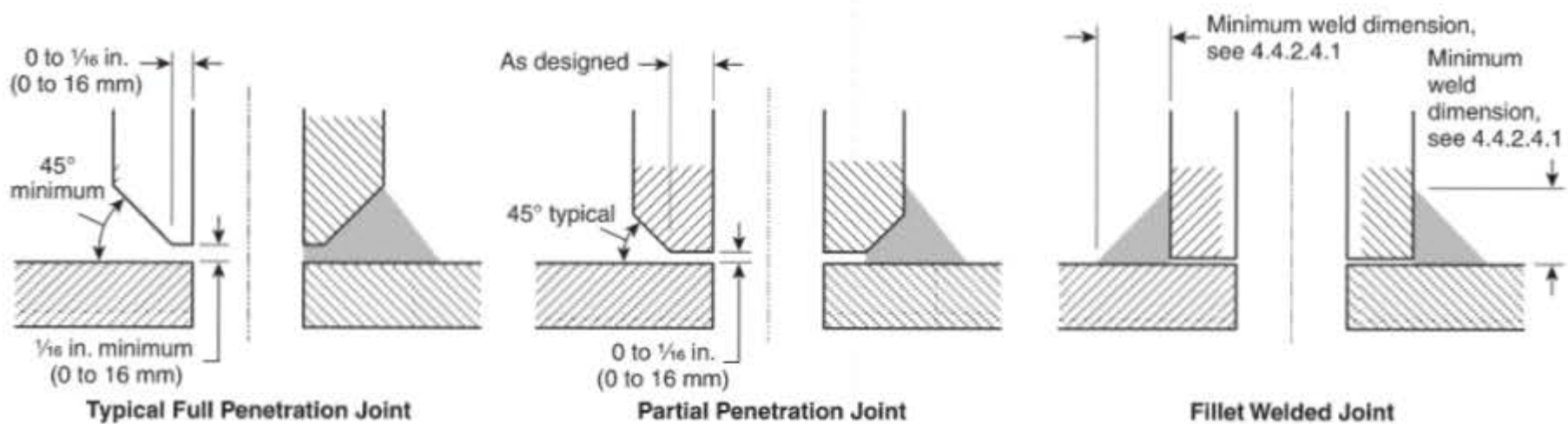
▲ FIGURE A.4.4.2.4.1 Weld Descriptions. [13:Figure A.7.5.2.4.1]
